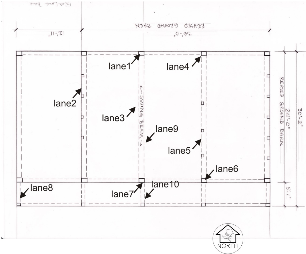
Figure 2. Floor plan of the Lane Barn showing sample locations on the first floor (base drawing compliments of Carla Cielo and the Holland Township Historic Preservation Commission).
