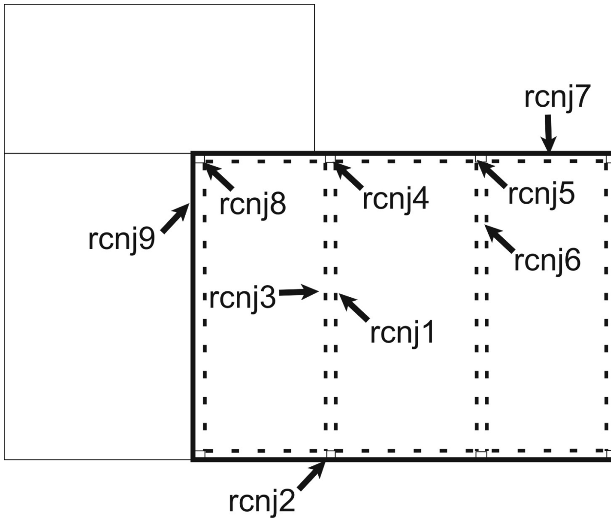
Figure 2. Sketch plan of Richard Cain Barn showing sample locations
